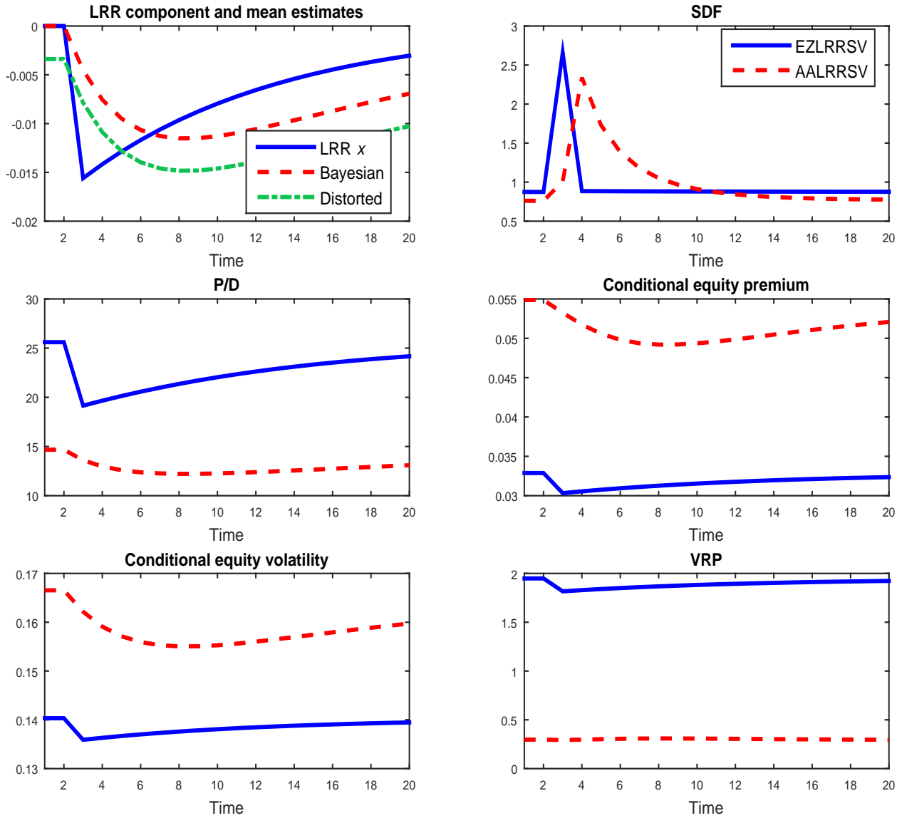
Figure 10: Impulse-response functions: AALRRSV and EZLRRSV
