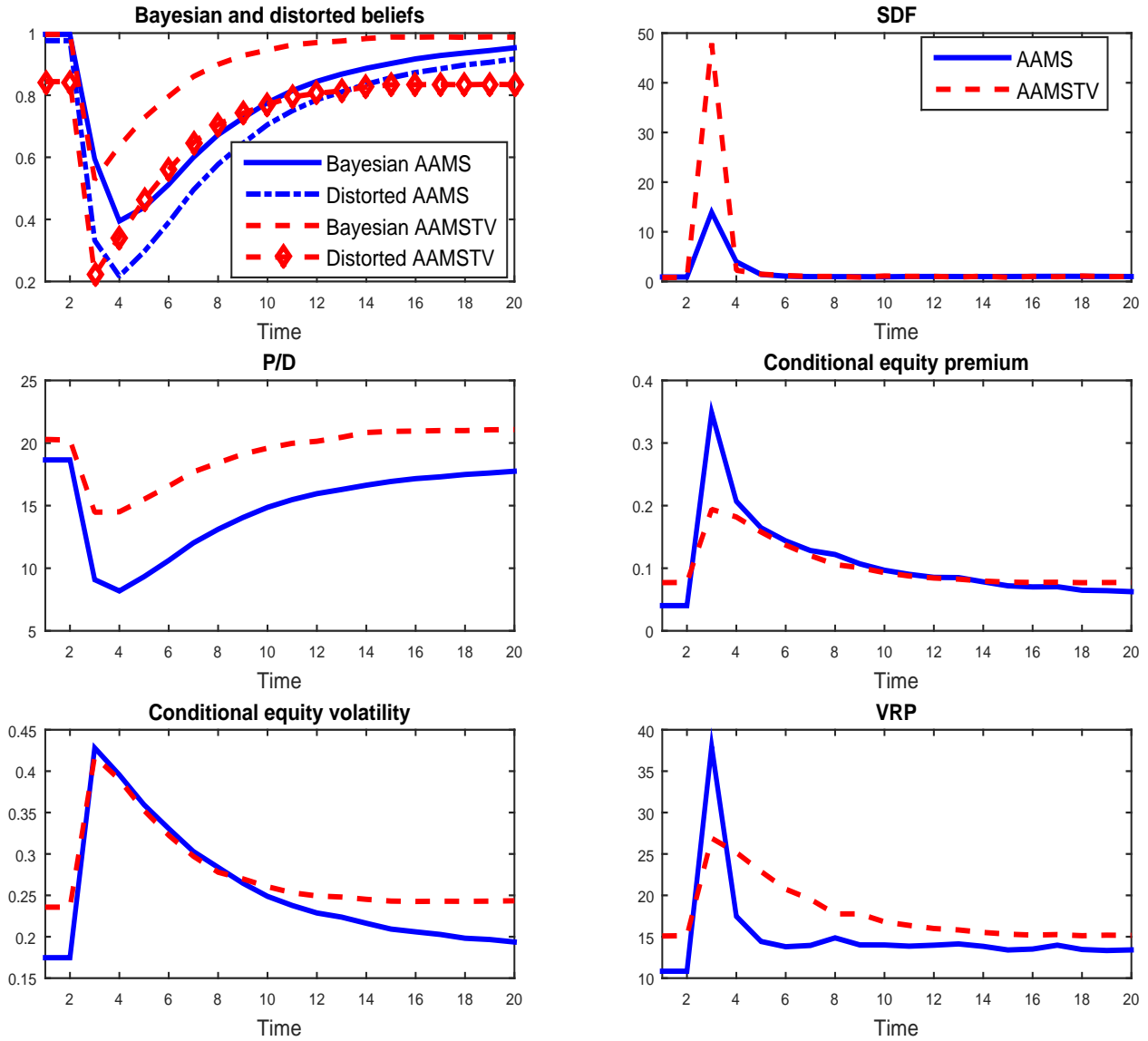
Figure 9: Impulse-response functions: AAMS and AAMSTV
