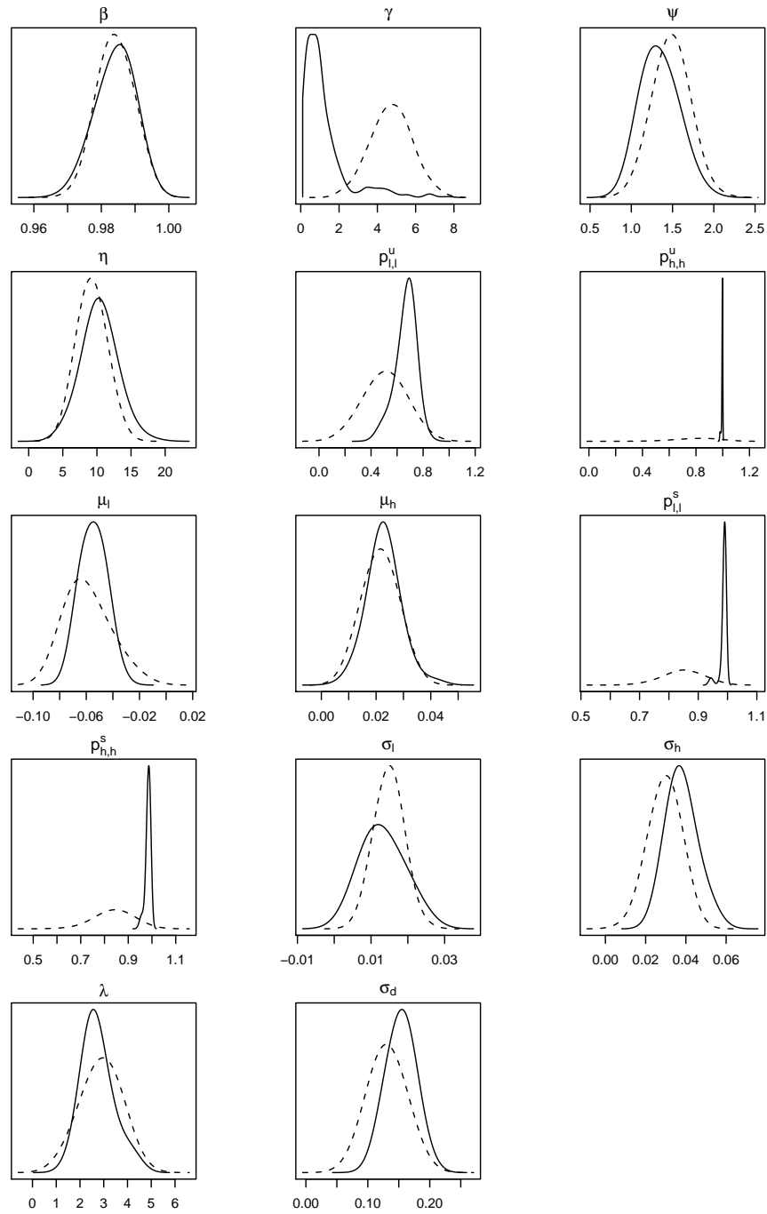
Figure 4: Prior and Posterior Densities of Estimated Parameters of AAMSTV Model
