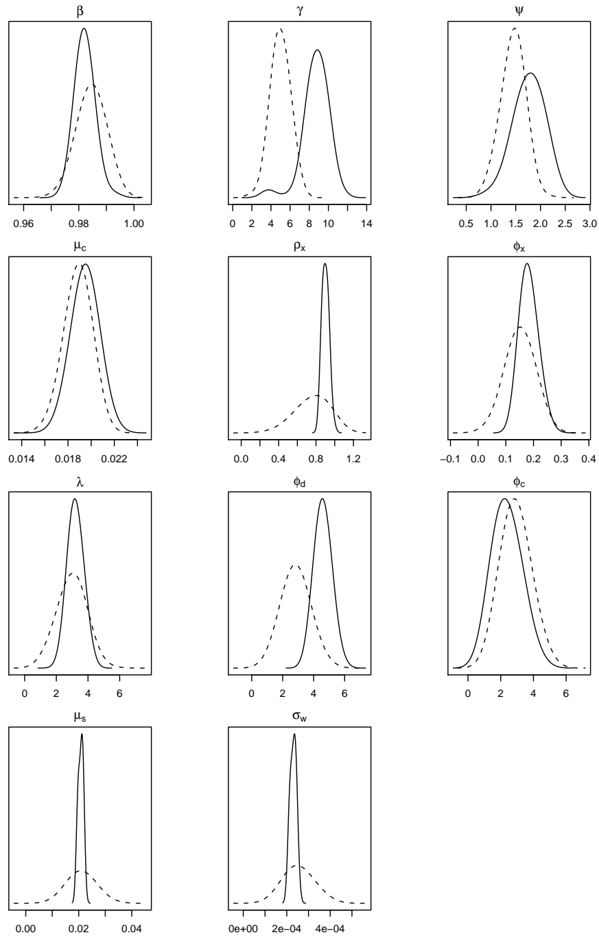
Figure 8: Prior and Posterior Densities of Estimated Parameters of EZLRRSV Model
