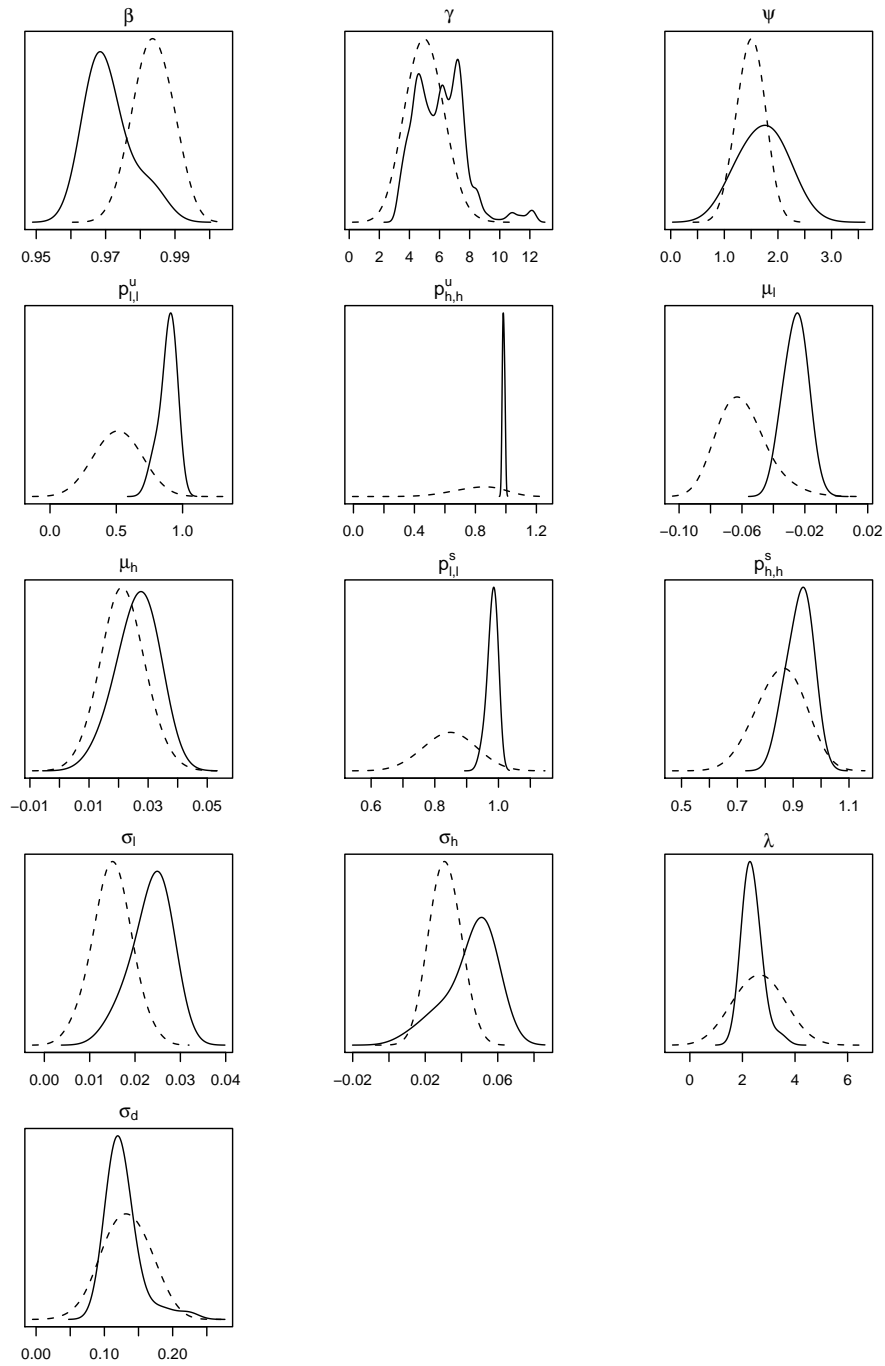
Figure 7: Prior and Posterior Densities of Estimated Parameters of EZMSTV Model
